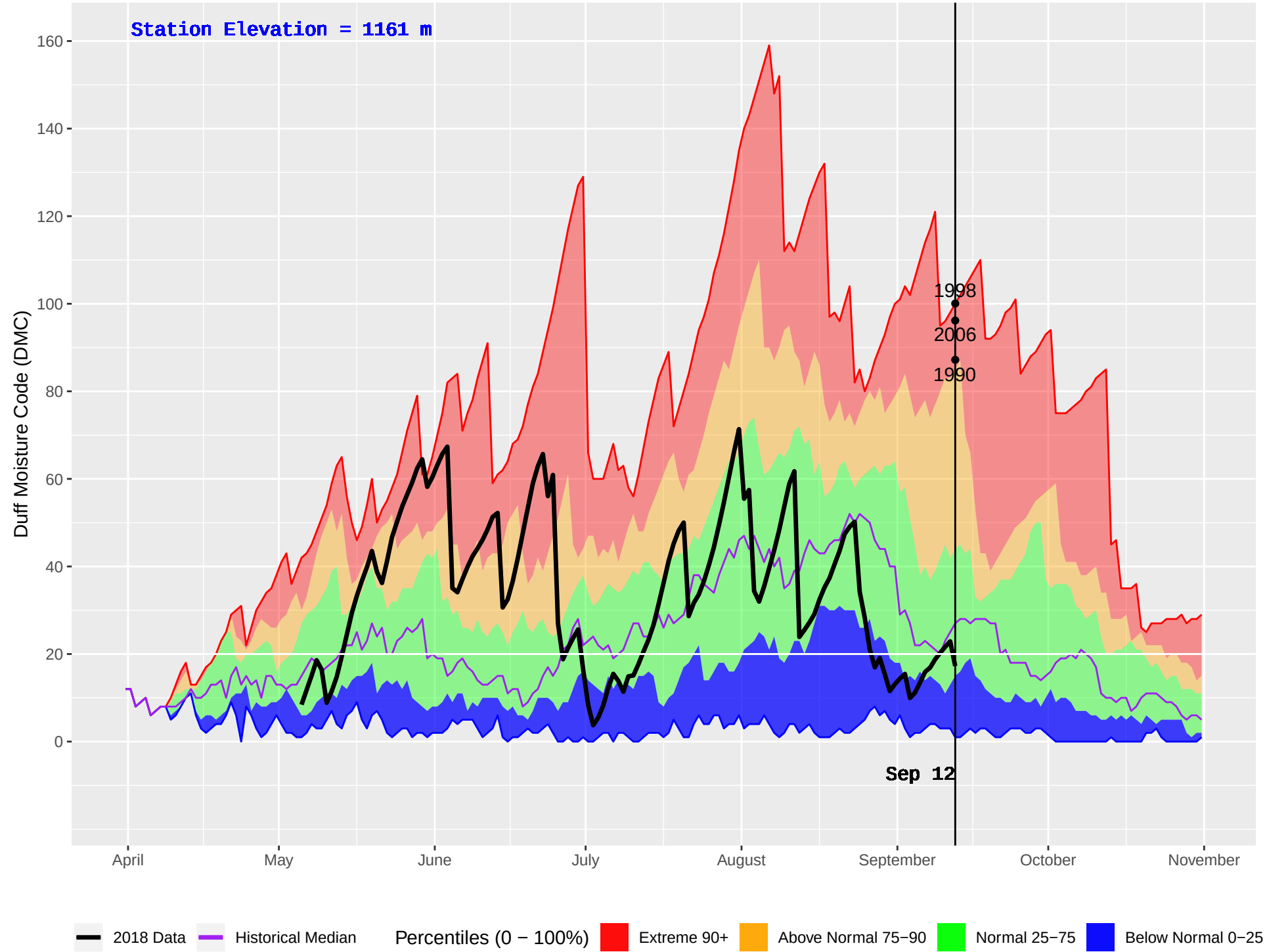
TIMOTHY (234) : Historical (1990–2016) and Current (2018) Daily Duff Moisture Code (DMC)
