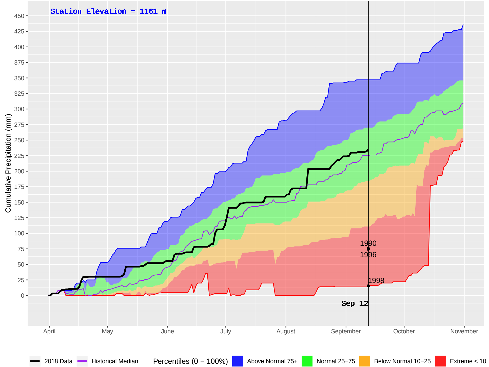
TIMOTHY (234) : Historical (1990–2016) and Current (2018) Daily Cumulative Precipitation
