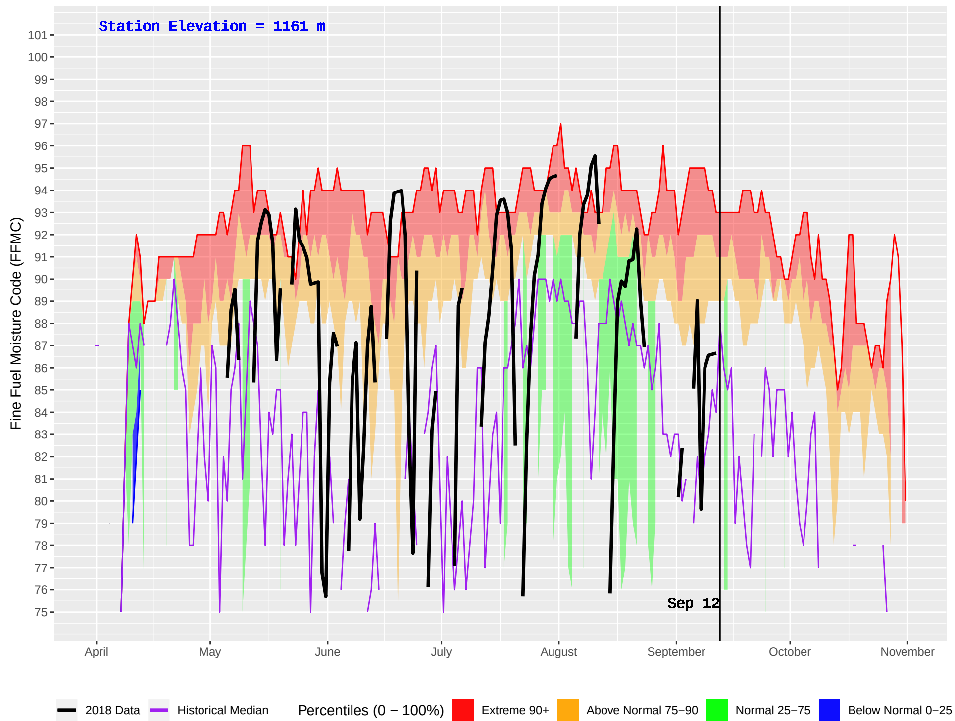
TIMOTHY (234) : Historical (1990–2016) and Current (2018) Daily Fine Fuel Moisture Code (FFMC)
