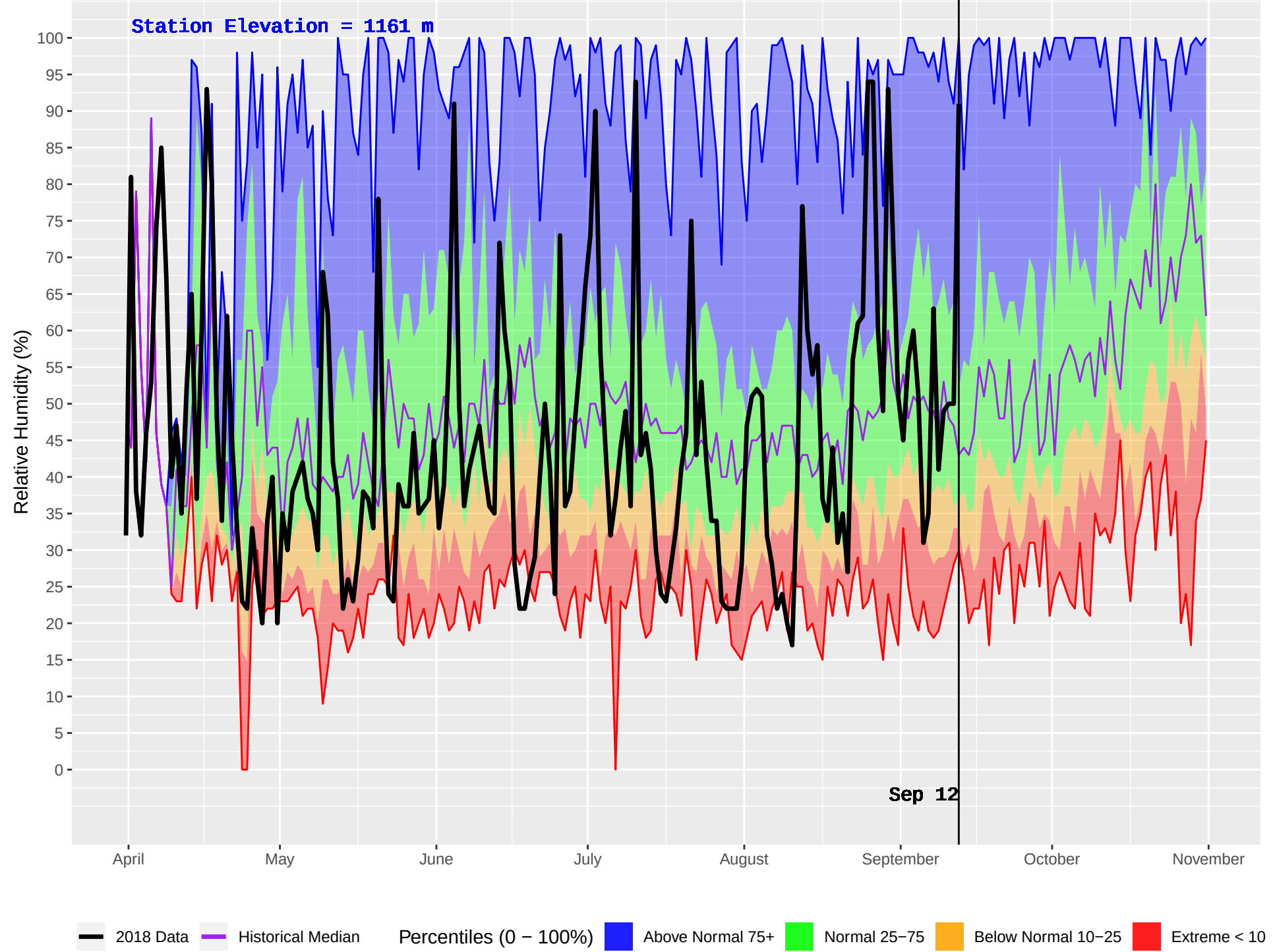
TIMOTHY (234) : Historical (1990–2016) and Current (2018) Daily Relative Humidity
