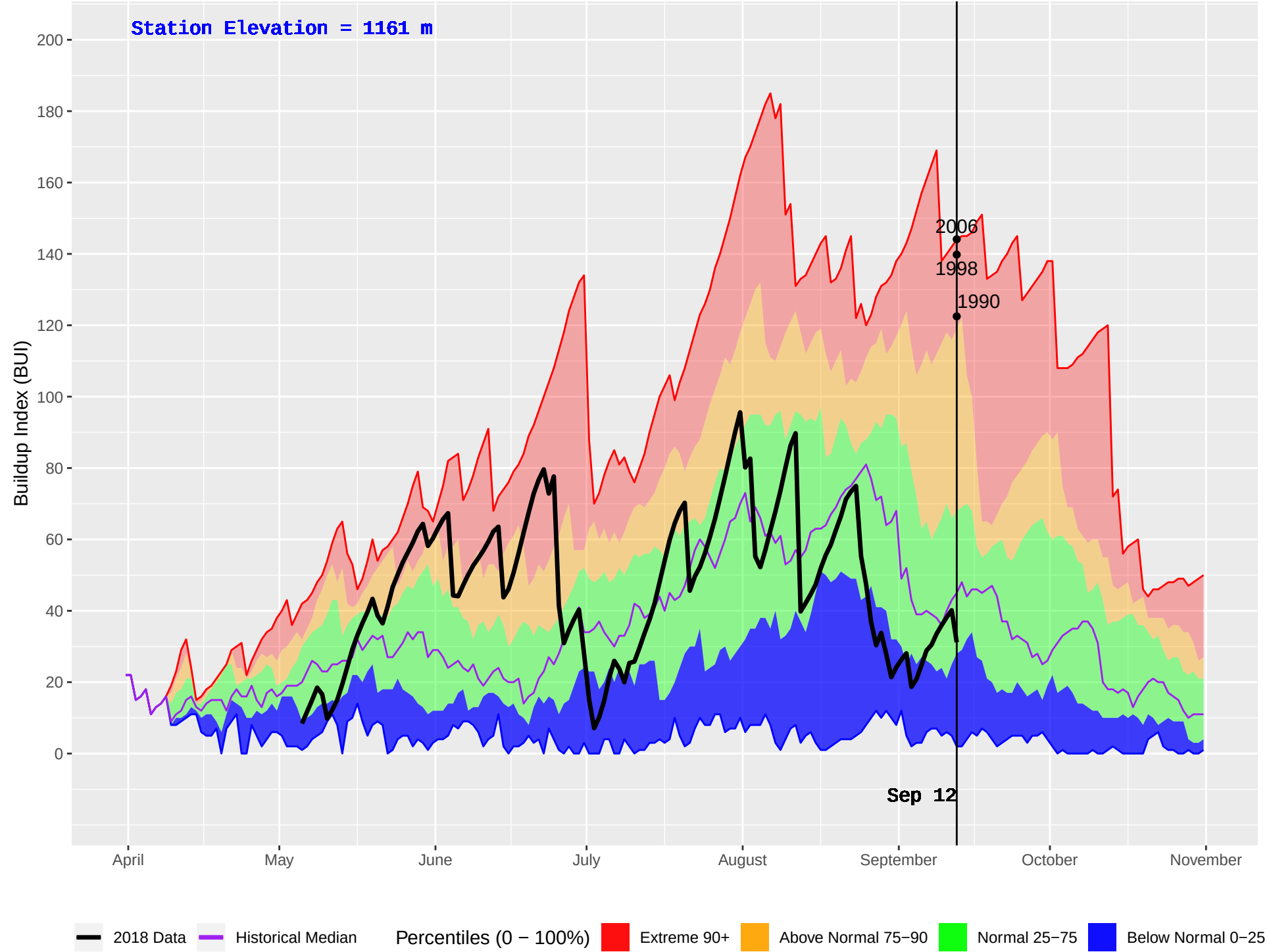
TIMOTHY (234) : Historical (1990–2016) and Current (2018) Daily Buildup Index (BUI)
